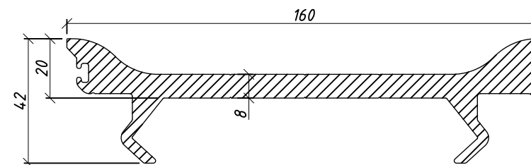
8-20/160 Leak Proof Deckslat HD-SEALED Artikelnr. : 862.7825
