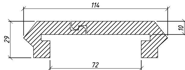
Plastic glider bearing T-subdeck LP Artikelnr. : 4107022.01 and 4107022.02
