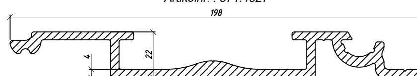
Alu 8/160 Leak Proof T subdeck (Turn-in) Artikelnr. : 871.4327
