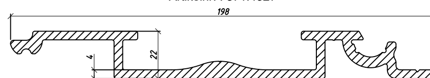
Alu 8/160 Leak Proof T subdeck (Turn-in) Artikelnr. : 871.4327
