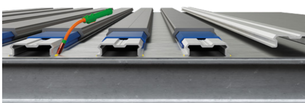
Loose aluminum subdeck profiles welded on an aluminum smooth plate.
