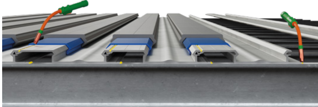
"Slide in" subdeck profiles welded on aluminum crossmembers (alternatively rivited), sealed by full length welds.
